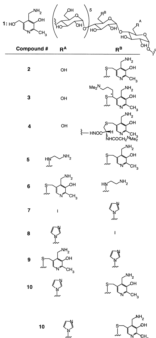
Figure 1. Pyridoxamine and pyridoxamine-cyclodextrin conjugates (and their precursors) evaluated as transaminase mimics. The lettering of glucose residues is clockwise and sequential A,B when the cyclodextrin is viewed from the primary face that carries the hydroxymethyl groups.
