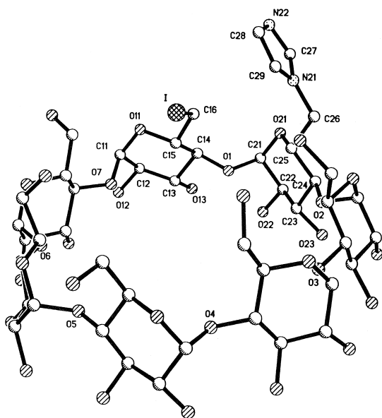
Figure 2. The crystal structure of compound 7 . The iodine is on the 6A position according to the convention and structure shown in Figure 1.
