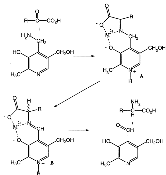
Scheme 1. Transamination of a ketoacid by pyridoxamine. In the compounds described in this paper, the CH 2 OH group is replaced by a CH 2 -S-cyclodextrin group.
